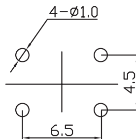
P. C. B. HOLE DETAIL
