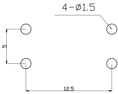
Mounting Dimensions
