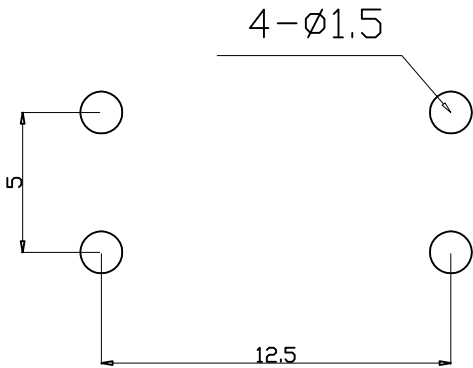
Mounting Dimensions
