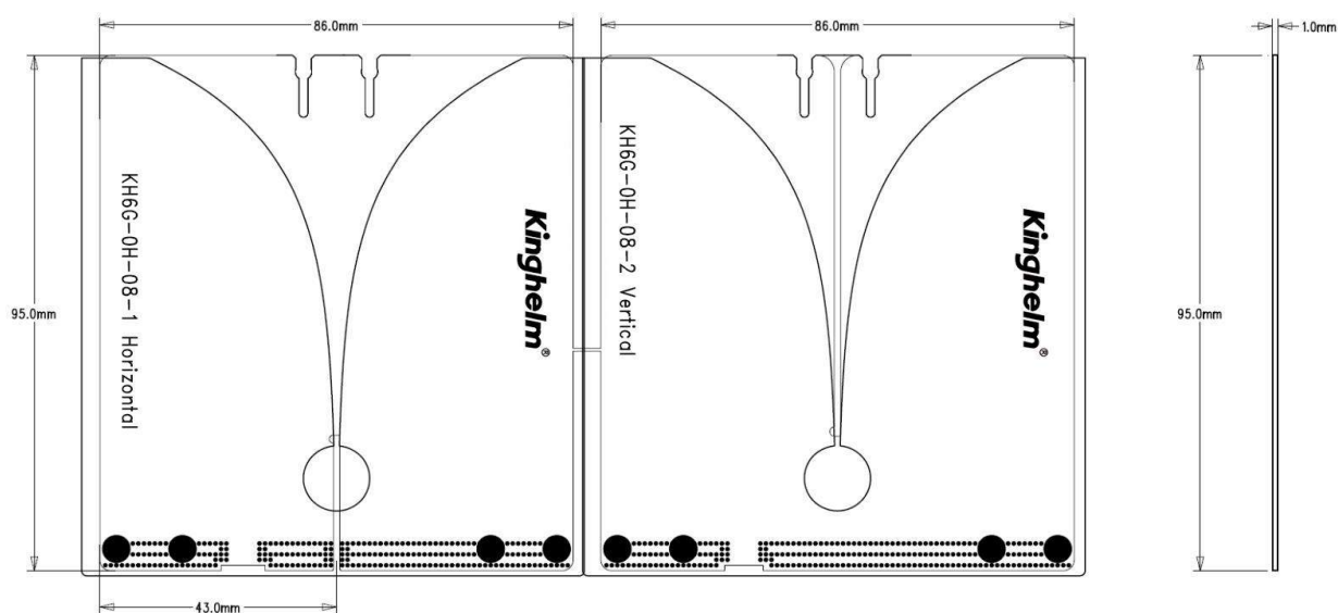
Figure1. KH-6G-0H-08 Geometry
