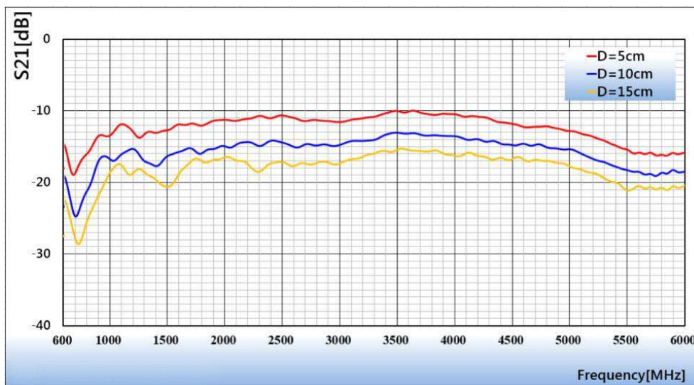
Graph2. KH-6G-0H-08 Path-Loss(Horizontal)
