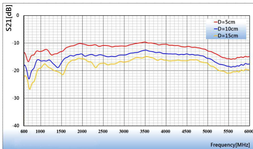
Graph3. KH6G-0H-08 Path-Loss(Vertical)
