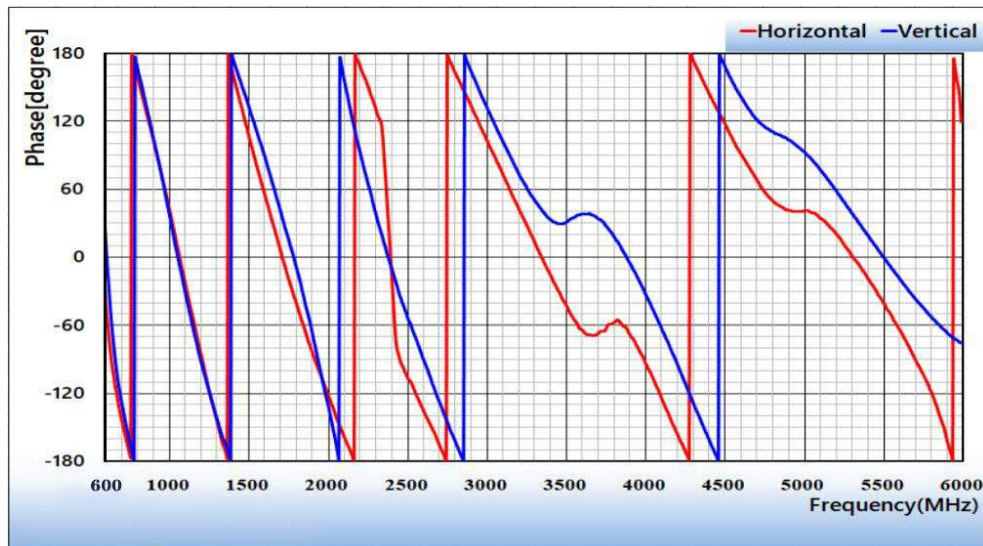
Graph4. KH-6G-0H-08 Phase
