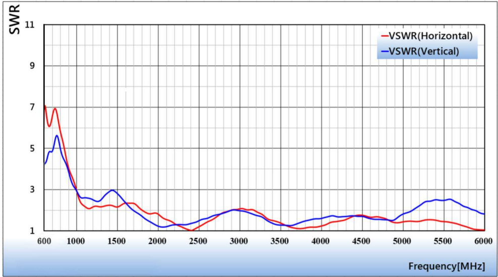
Graph1. KH6G-0H-08 VSWR
