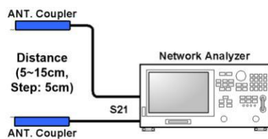
Figure2. Test Setup
