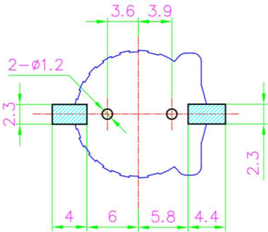
PCB Holes Diagram Top View
